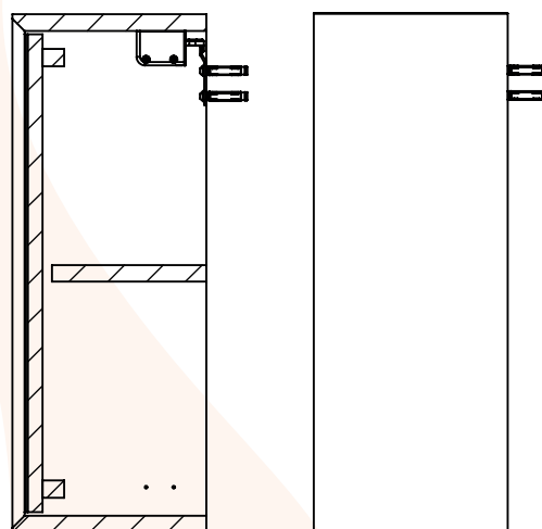
SECTION K-K
